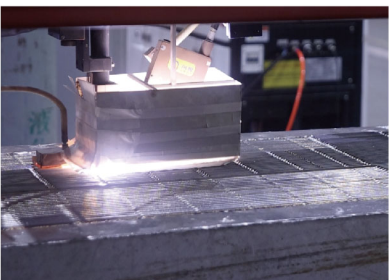
Automatic plate welding (AWD, A-bloc)
